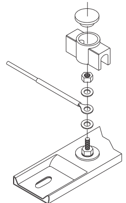
Ceramic Cap Thread 10-32 Part Number CER-102-101
